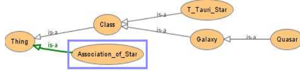
Fig. 5. Final ontology
