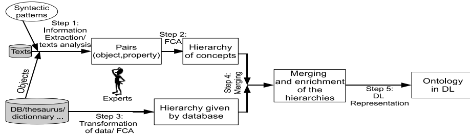
Fig. 1. PACTOLE Methodology
