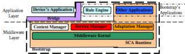
Figure 1. Middleware Platform Architecture
