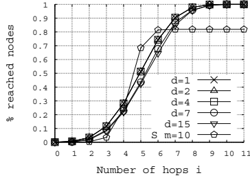
(a) Number of nodes N = 2000
