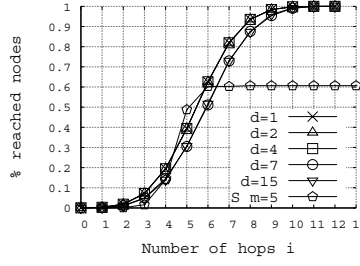
(b) Number of nodes N = 5000
