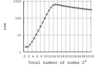
Fig. 8. Impact of attacks - res(n)
