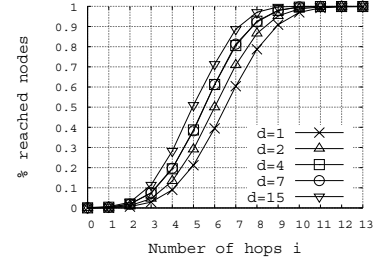
(c) Identifier space size N_{MAX} = 2^{14}
