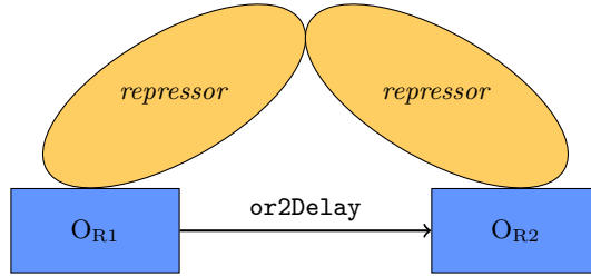
Fig. 9. The decay of the repressor - \text{OR}_2 complex: in order to make the decay rate of the repressor - \text{OR}_2 complex dependent on \text{OR}_1 ’s state, the two sites communicate on or2Delay before \text{OR}_2 unbinds.
