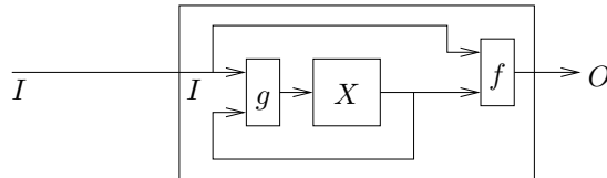
Figure 5: An equational view of a reactive system
