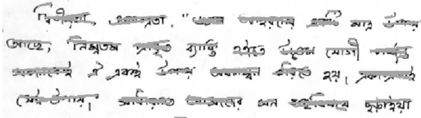
(b) Resolution -8
