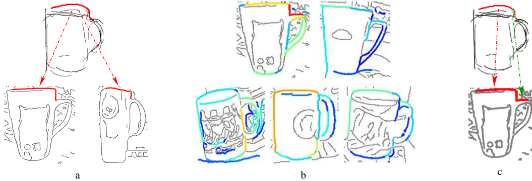
Figure 5: Occurrences and connectedness. a) A model part (above) and two of its occurrences (below). b) All occurrences of all model parts on a few training images, colored by their confidence (increasing from blue to cyan to green to yellow to red). c) Two model parts with high connectedness (above) and two of their occurrences, which share a common segment (below).
