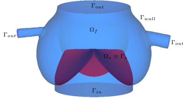
Figure 11: Computational domain.
