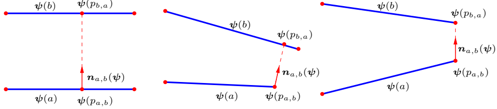
Figure 6: Possible configurations of the unit vector \mathbf{n}_{a,b}(\psi) .
