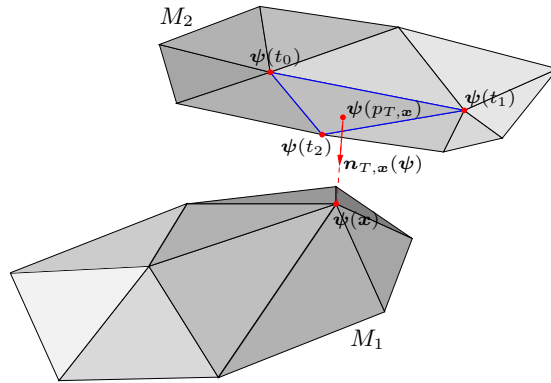
Figure 7: Computation of the unit vector \mathbf{n}_{T,x}(\psi) for the triangle/vertex couple (T, x) .
