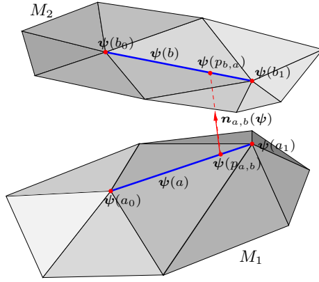
Figure 5: Computation of the unit vector \mathbf{n}_{a,b}(\psi) for the edge/edge couple (a, b) .
