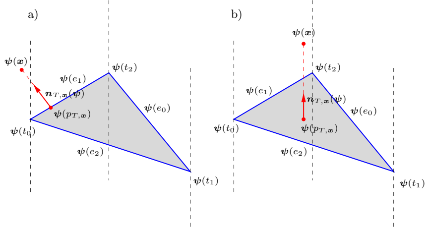
Figure 8: Possible configurations of the unit vector \mathbf{n}_{T,x}(\psi) . a) \psi(x) is in the part of the space opposed to \psi(t_1) with respect to the plane that contains \psi(e_1) . b) \psi(x) is inside the cylinder determined by the intersection of the three perpendicular planes to \psi(T) .
