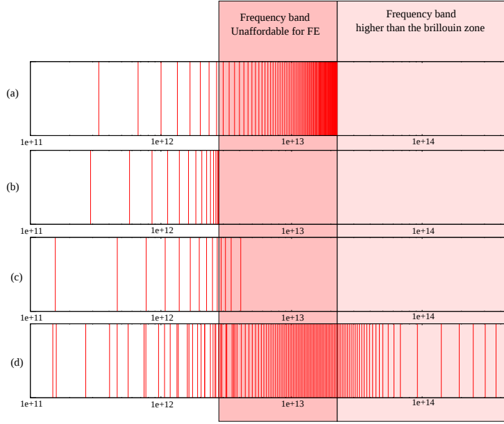
Figure 13: Spectrum of a monoatomic chain constituted of 104 atoms (a), of a 1D homogeneous grid with finite element size of h = 8r_0 (b), and of the coupling model in its complete (c) and its condensed form (d).
