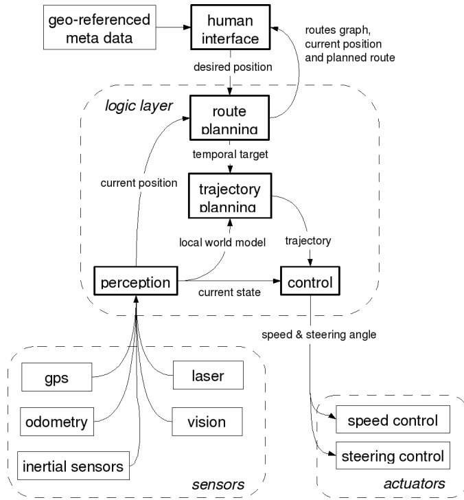
Figure 5. Logic diagram of the system
