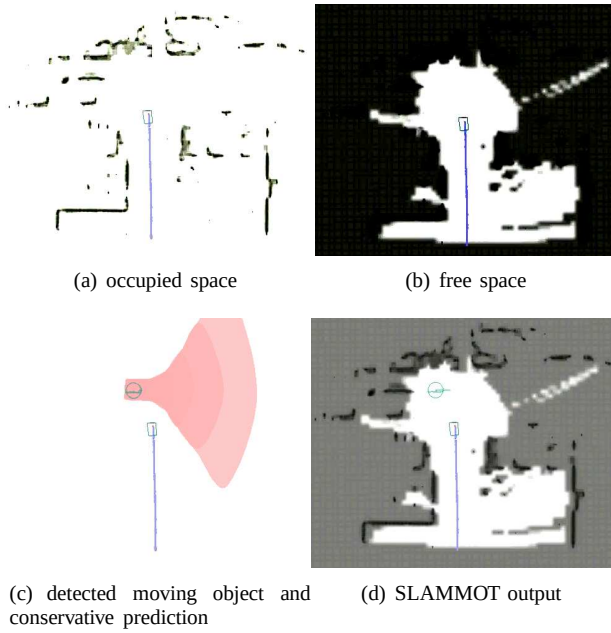
Figure 1. Different components of our SLAMMOT algorithm internal representation and final output
