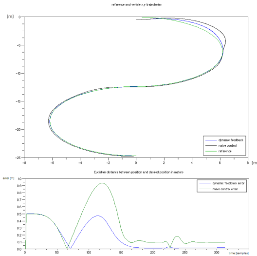
Figure 4. Comparison of the naive and dynamic feedback controllers on an error free situation. The later performs notoriously better
