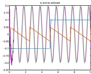
Fig. 5. Unknown input and estimation (nominal case)
