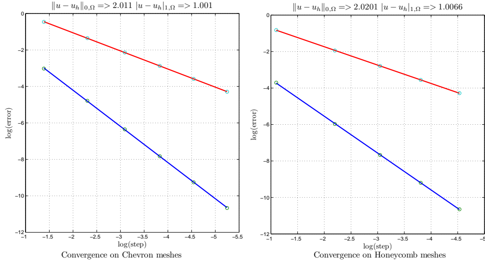
Figure 5: Convergence curves when P_K = Q_1^K
