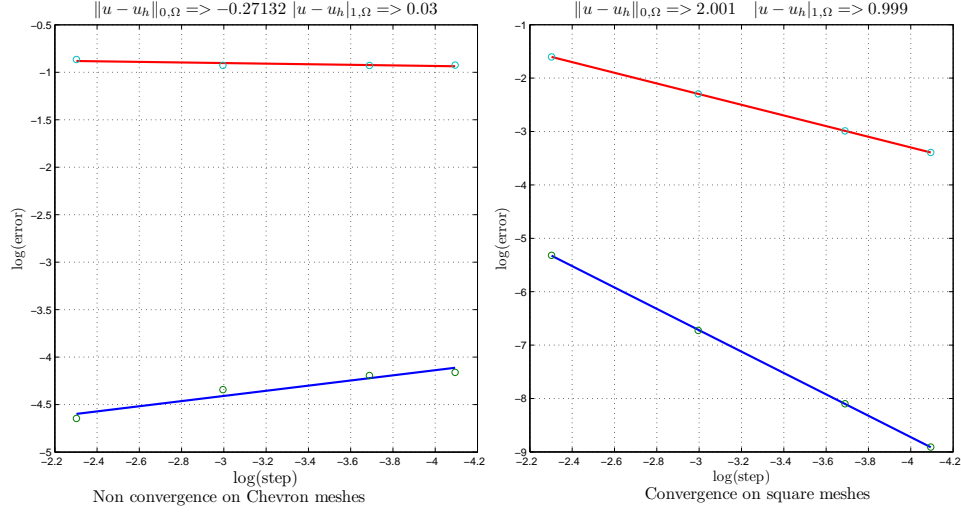
Figure 5: Convergence curves when P_K = Q_1^K
