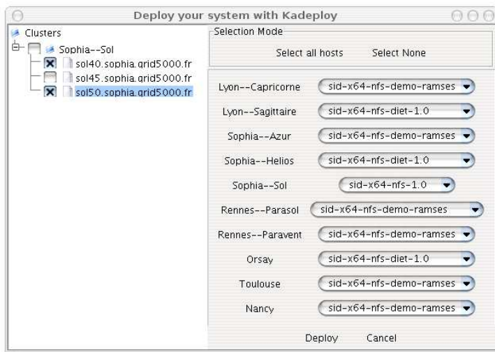
Figure 3: Image deployment through KaDeploy.
