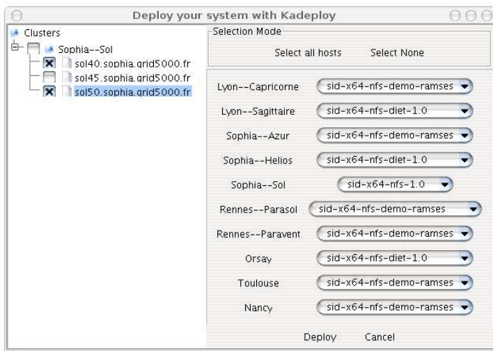
Figure 3: Image deployment through KaDeploy.
