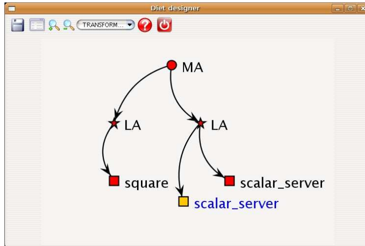
Figure 6: DIET designer.
