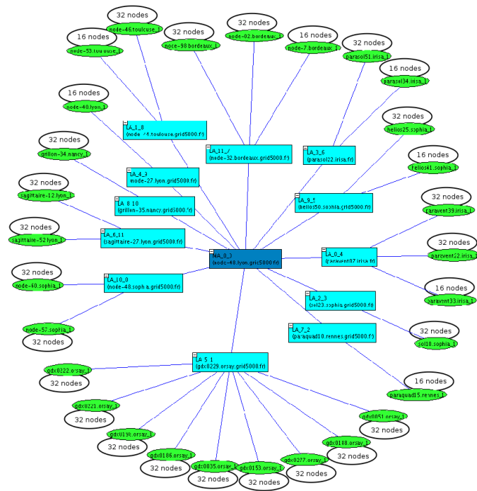
Figure 10: DIET hierarchy deployed during the experiment.
