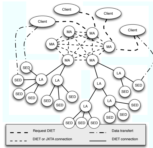
Figure 1: DIET hierarchical organization.
