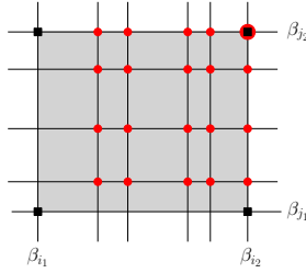
Figure 4: The sum of the multiplicities of the nodes (red disks) contained in the box (\beta_{i_1}, \beta_{i_2}] \times (\beta_{j_1}, \beta_{j_2}] is equal to the alternate sum of the ranks of the linear maps corresponding to the vertices (black squares) of the box.
