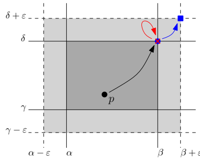
Figure 7: Possible images of p \in D\mathcal{F}_\mathbb{R} \cap \square through the multi-bijection m_4^{-1} \circ m_3 \circ m_2^{-1} \circ m_1 : m_1(p) is the blue disk with coordinates (\beta, \delta) ; m_2^{-1} \circ m_1(p) is the red cross that coincides with the blue disk; m_3 \circ m_2^{-1} \circ m_1(p) is the blue square; m_4^{-1} \circ m_3 \circ m_2^{-1} \circ m_1(p) is located in the light gray box \square_\varepsilon .
