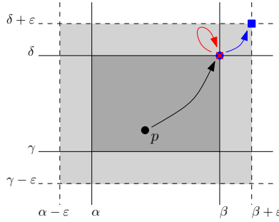
Figure 7: Possible images of p \in D\mathcal{F}_\mathbb{R} \cap \square through the multi-bijection m_4^{-1} \circ m_3 \circ m_2^{-1} \circ m_1 : m_1(p) is the blue disk with coordinates (\beta, \delta) ; m_2^{-1} \circ m_1(p) is the red cross that coincides with the blue disk; m_3 \circ m_2^{-1} \circ m_1(p) is the blue square; m_4^{-1} \circ m_3 \circ m_2^{-1} \circ m_1(p) is located in the light gray box \square_\varepsilon .
