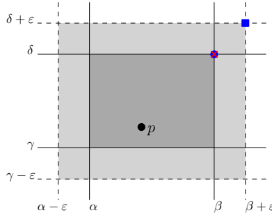
Figure 7: Possible images of p through the multi-bijection m_4^{-1} \circ m_3 \circ m_2^{-1} \circ m_1 : m_1(p) is the blue disk with coordinates (\beta, \delta) ; m_2^{-1} \circ m_1(p) is the red cross that coincides with the blue disk; m_3 \circ m_2^{-1} \circ m_1(p) is the blue square; m_4^{-1} \circ m_3 \circ m_2^{-1} \circ m_1(p) is located in the light gray box B_\varepsilon .
