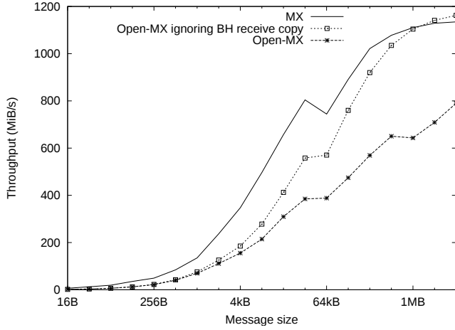
Fig. 3. Expected Open-MX performance improvement when removing the copy in the receive callback (invoked by the bottom half interrupt handler of the driver).
