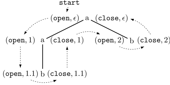
Fig. 1. The total ordering on events(a(a(b), b))
