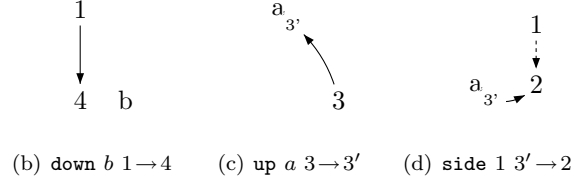
Fig. 6. Run of a PFA
