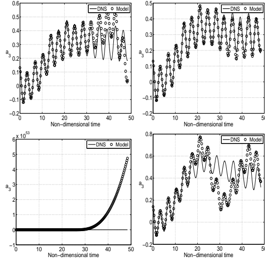
FIG. 5 – a_3 DNS (continuous line) with K = 0.8 (top) and K = 1.3 (bottom) versus a_3 obtained when the model is calibrated with \alpha = 1.6 \times 10^{-6} (left) and when \alpha = 10^{-3} (right)
