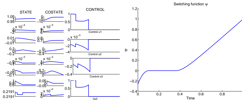
Goddard (3D) - State, costate, control and switching function
