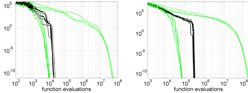
Fig. 2. Simulation of \text{AE}_{\text{CMA}}-(1, \lambda) -Cauchy-ES (bold) and (1, \lambda) -Cauchy-ES (light) on the axisparallel (solid) and the rotated (dashed) f_{\text{elli}} in 10-D (left) and 30-D (right). Shown is the objective function value of respectively 3 trials over time. In the rotated case, the \text{AE}_{\text{CMA}} improves the performance by a factor of roughly one thousand.
