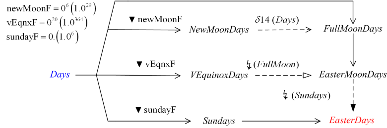
Figure 8: Clock dependency graph for Easter
