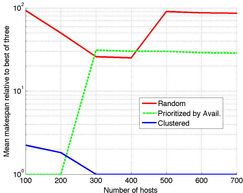
Figure 6: Performance of Barrier Synch Application
