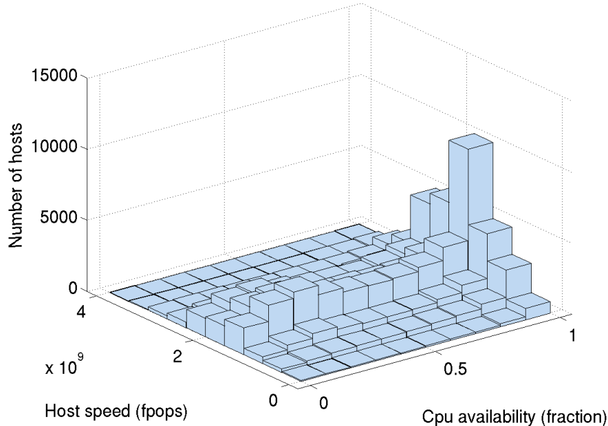
Figure 2: Distribution of host speeds versus CPU availability
