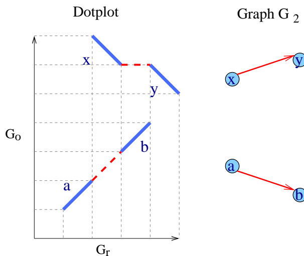
Figure 3: Example of a conflicting arc of type II. On the left-hand side is a dotplot representation of the positions of anchors a , b , x and y on the G_r and G_o . Anchors a and b are on the same chromosome in the two genomes and d(a, b) = 2 , the same for x and y . On the right-hand side is the corresponding graph \mathcal{G}_2 ( k = 2 ). It has two connected components: \{a, b\} and \{x, y\} . The arc ab is conflicting because a_r < x_r < b_r and x belongs to another component with at least two anchors.
