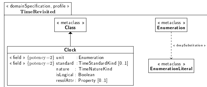
Figure 6: Choice of extended metaclasses.
