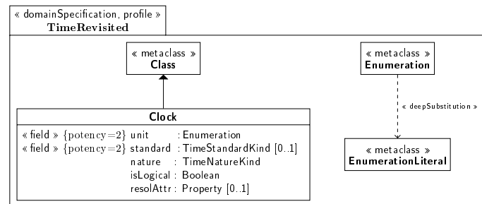
Figure 6: Choice of the extended metaclasses.
