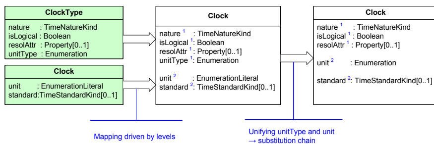
Figure 3: Clock definition with potency information
