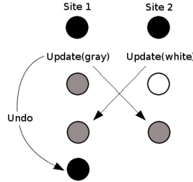
Figure 1: Undo in a graphical editor
