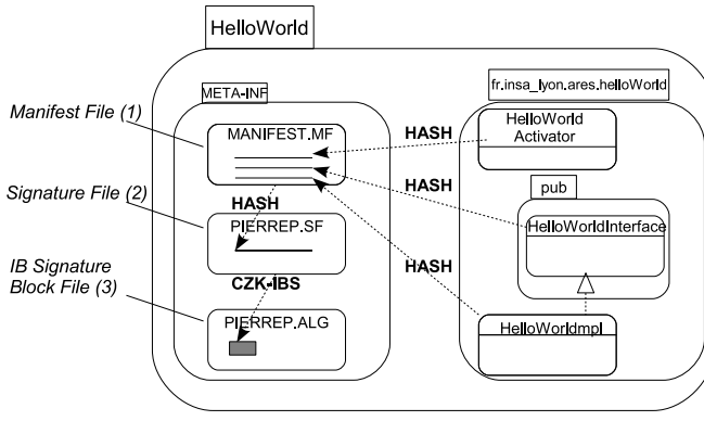
Figure 3. Structure of a signed bundle, using Identity-based Cryptography
