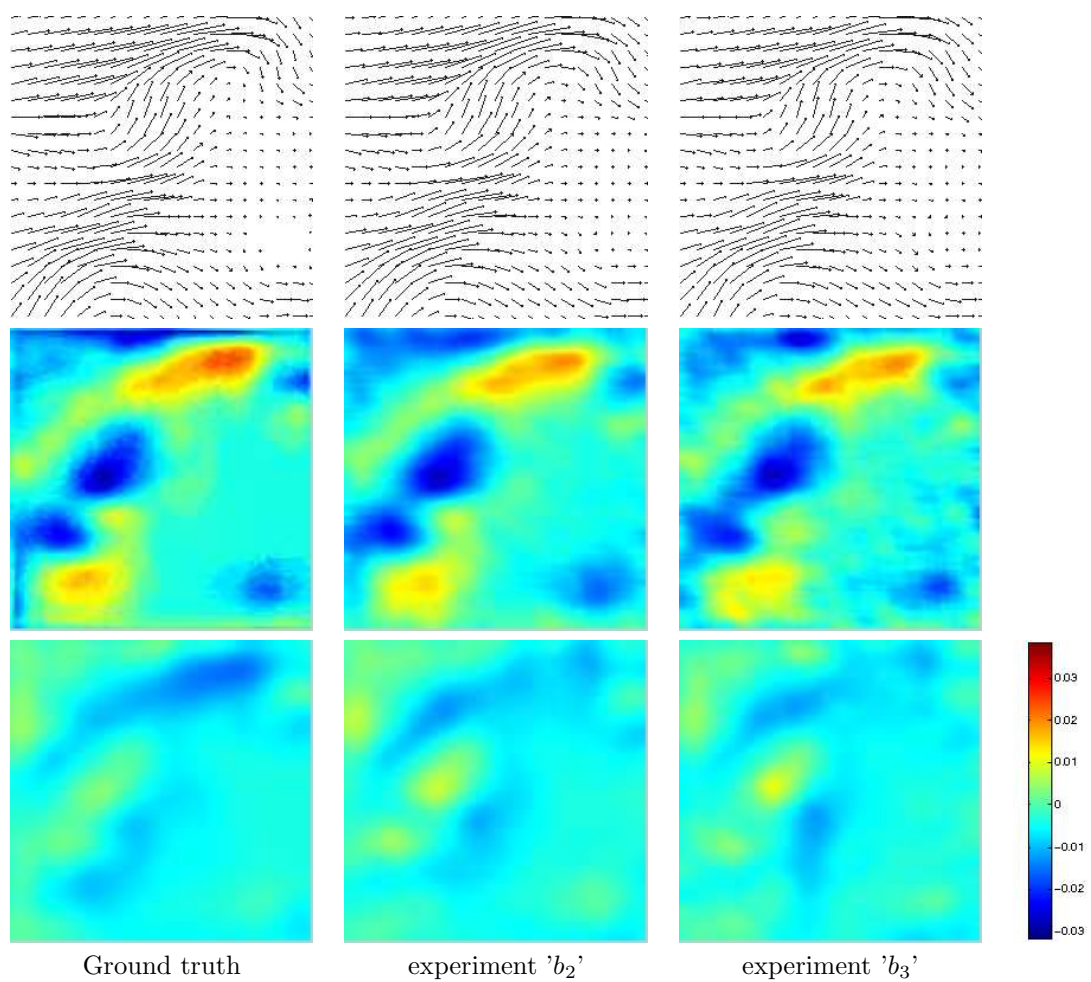
Figure 10: Variables after assimilation with an imperfect model : Wind \tilde{\mathbf{v}}^k (first line), vorticity \tilde{\zeta}^k (second line) and divergence \tilde{D}^k (third line) fields at t=1h15min
