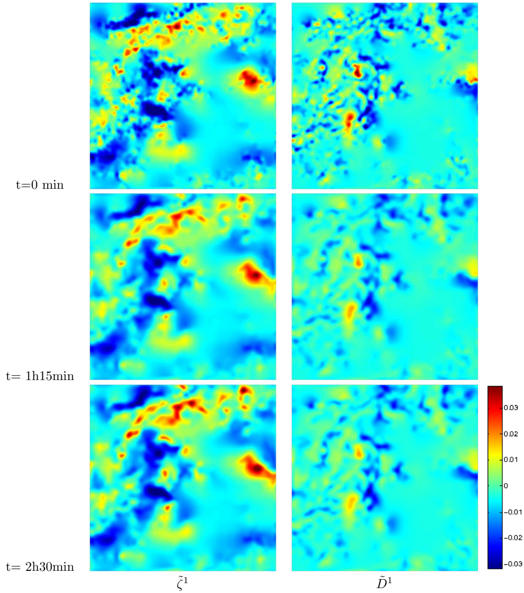
Figure 16: Vorticity and divergence estimated by assimilation with imperfect modeling. Divergence \tilde{D}^1 and vorticity \zeta^1 of the lower layer at different times.
