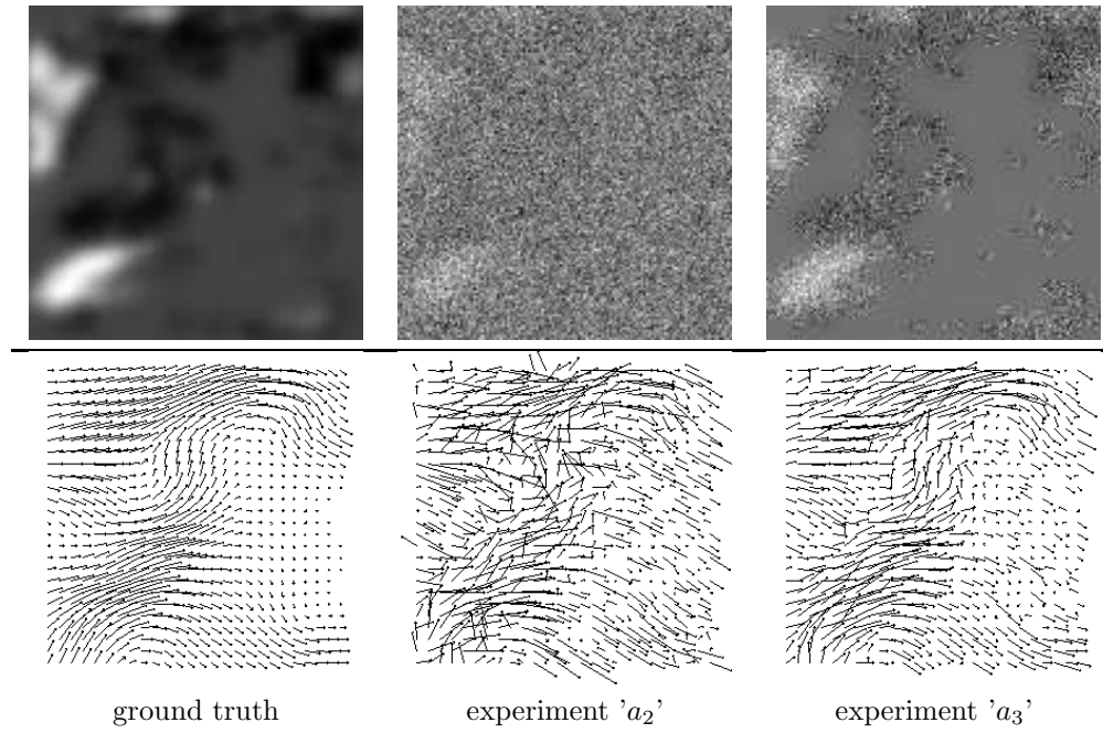
Figure 5: Observations and state variables before assimilation with a perfect model : \tilde{h}_{obs}^k(t_0) (first line) and \tilde{v}^k(t_0) (second line) at initial time.
