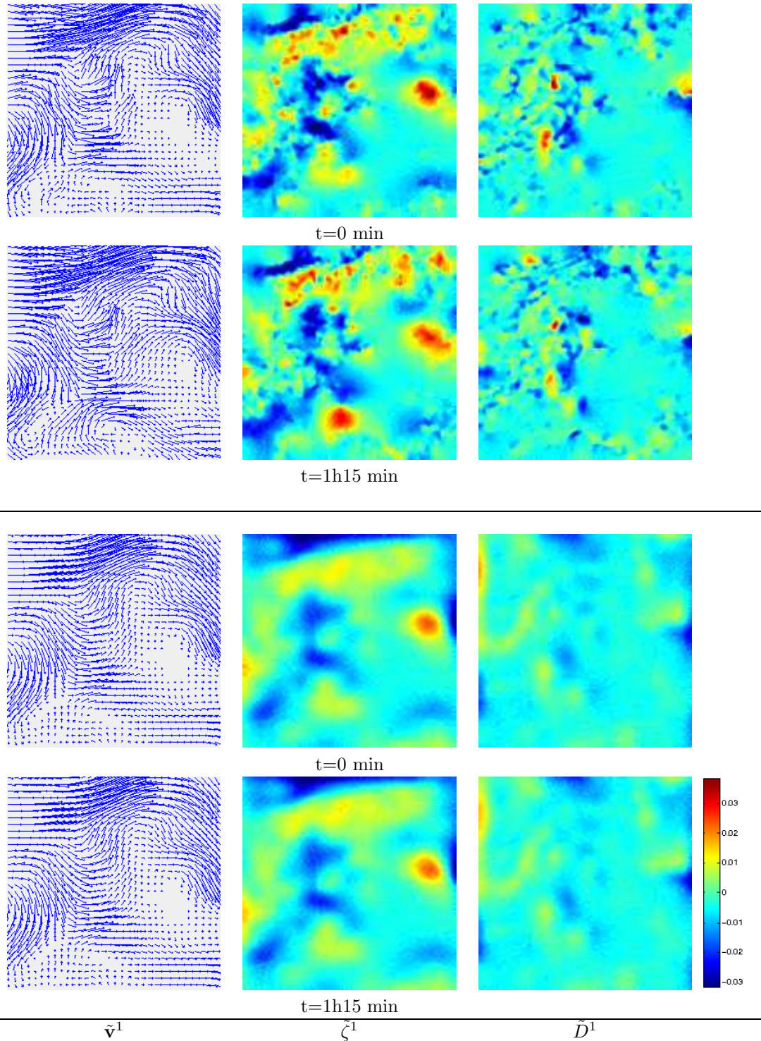
Figure 13: Comparison of a reference optic-flow method (two first lines) with assimilation with perfect modeling (two last lines) . Divergence \tilde{D}^1 , vorticity \tilde{\zeta}^1 and wind \tilde{v}^1 of the lower layer estimated by a reference optic-flow method and by assimilation with a perfect model.
