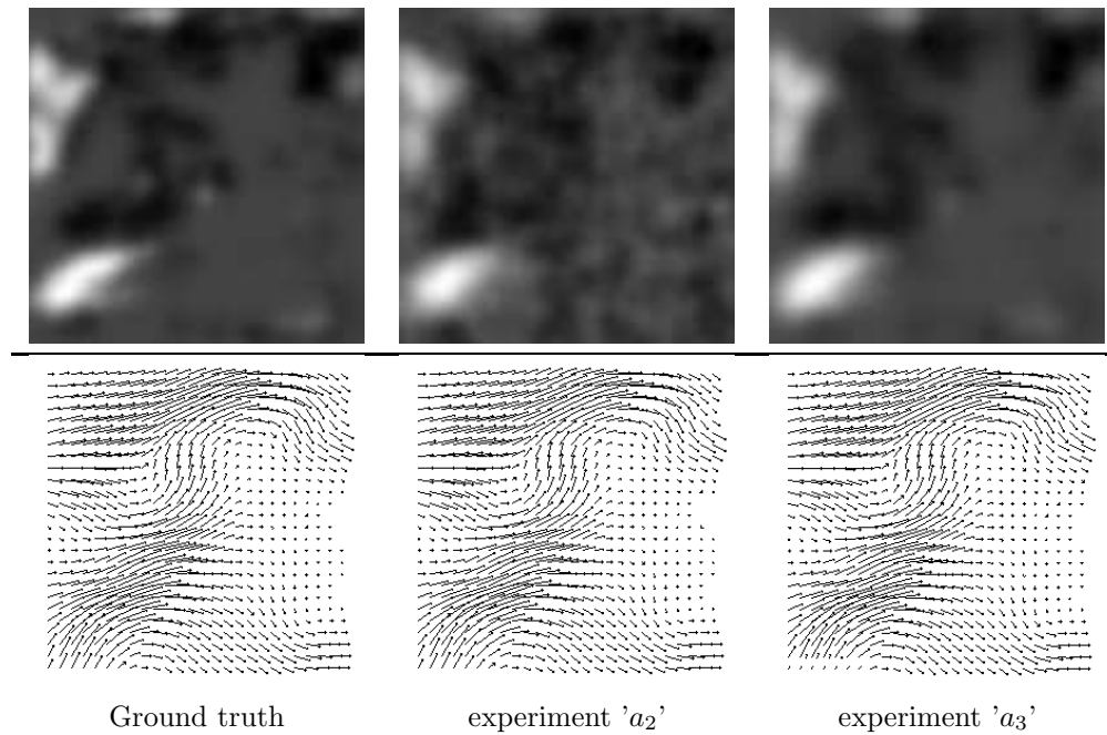
Figure 6: Variables after assimilation with a perfect model : pressure difference \tilde{h}^k(t_0) (first line) and wind fields \tilde{v}^k(t_0) (second line) estimates at initial time.
