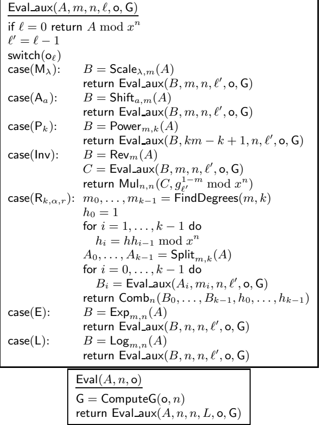
Figure 1: Algorithm Eval.
