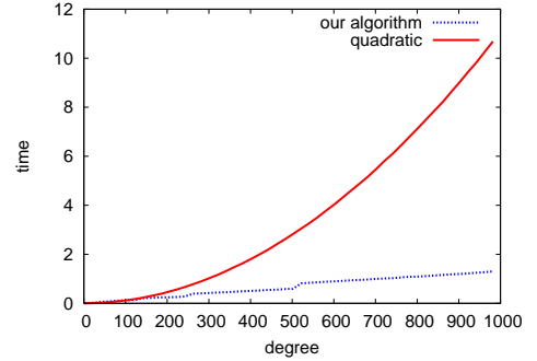
Figure 3: Jacobi polynomials.
