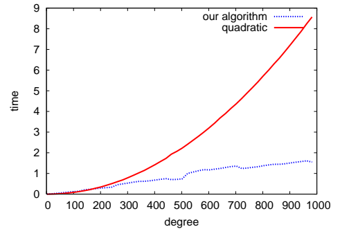
Figure 4: Mittag-Leffler polynomials.
