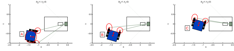
Fig. 3. Docking trial simulation illustrating controller course-correction to eliminate gross y -position errors. At position C, the wheelchair switches to path-following mode for final docking. In this example, \theta_{max} = 75^\circ .
