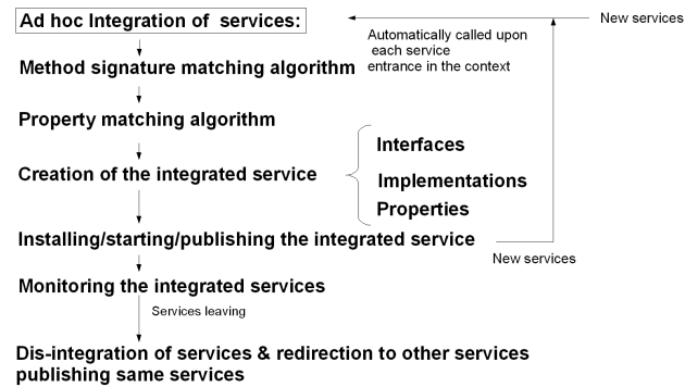
Fig. 7. automatic integration life cycle
