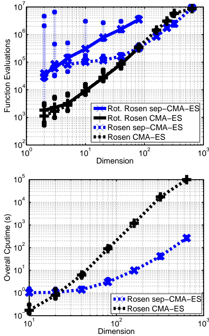
Figure 8: Results of sep-CMA-ES on the Rosenbrock function (in dashed line, rotated Rosenbrock function in plain line) compared to CMA-ES. Lines show median of the distribution, vertical error-bars show minimum and maximum number of evaluations on successful runs out of 11 runs on smaller dimension, 2 runs on larger dimension. Target function value is 10^{-9} .
