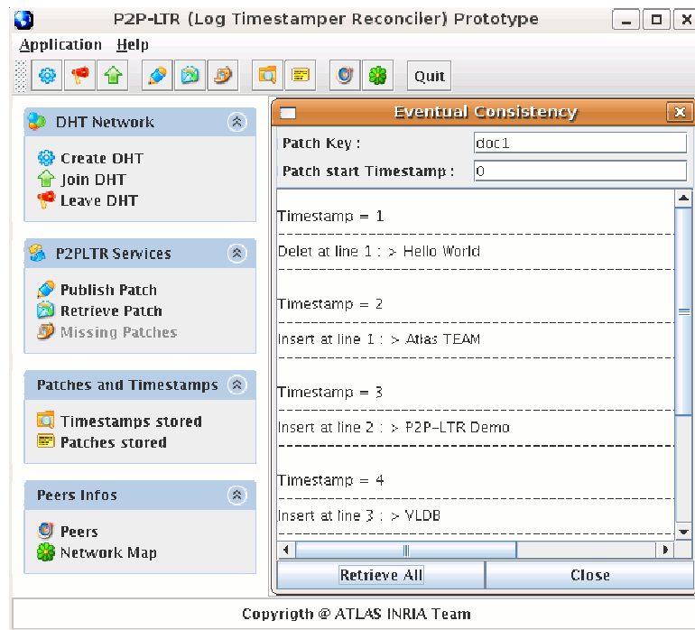
Figure 5. Missing patches retrieval on total order
