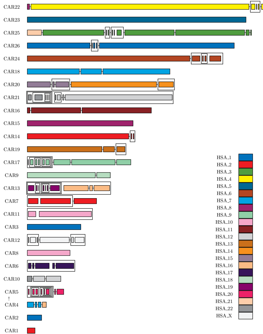
Figure 5: The ancestral genome architecture obtained with the dataset constructed from the UCSC whole genome alignments, with parameters max\_gap = 100\text{kb} and min\_len = 400\text{kb} . Segments of a given color represent sequences of genomic markers that are colinear in the inferred CARs and in a human chromosome (colors correspondences are given in the bottom right part of the figure), called conserved segments . There are 111 such conserved segments. The size of conserved segments in the figure is proportional to the sum of the sizes, in the human genome, of the synteny blocks they contain. The nodes of the PQ-tree are represented: children of a linear (Q) node are linked by a small segment, while children of a prime (P) node are grouped together with a rectangular frame.
