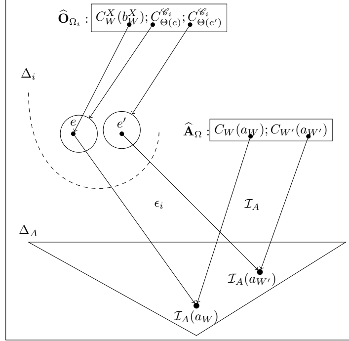
Figure 2: Construction of \epsilon_i from \mathcal{I}_i and \mathcal{I}_A . For each e = \mathcal{I}_i(b_W^X) or e \in \mathcal{I}_i(C_{\Theta(e)}^{\mathcal{C}_i}) we can find an individual a_W in \widehat{\mathbf{A}}_{\Omega} such that \epsilon_i(e) is assigned to \mathcal{I}_A(a_W) .
