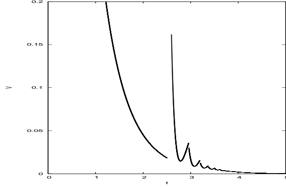
Figure 2: Typical evolution of the Lyapunov function during one cycle of a weakly stable system.
