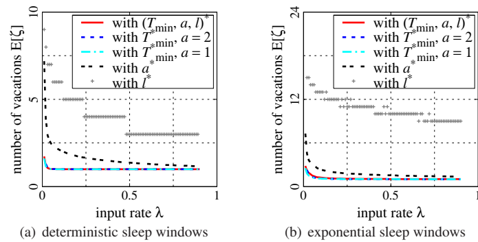
Figure 11: Expected number of vacations E[\zeta] versus \lambda when the protocol parameters are optimally set.
