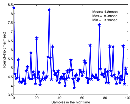
Fig. A.3. The RTT in the nighttime between the two PCs by Internet (40km away).
