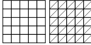
FIG. 7 – Square grid mapped into the triangular grid
