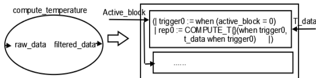
Figure 9: A simple subprogram mapping example
