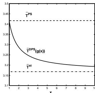
Figure 1: \bar{T}^{DPS}(g(x)) , \bar{T}^{PS} , \bar{T}^{st} functions.
