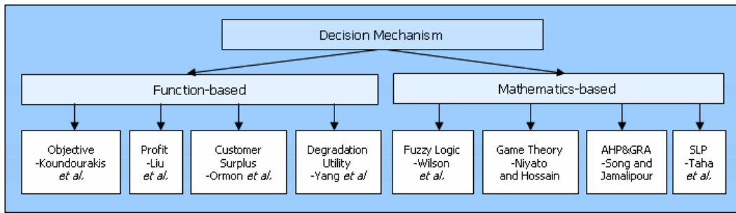
Figure 4: Decision mechanism
