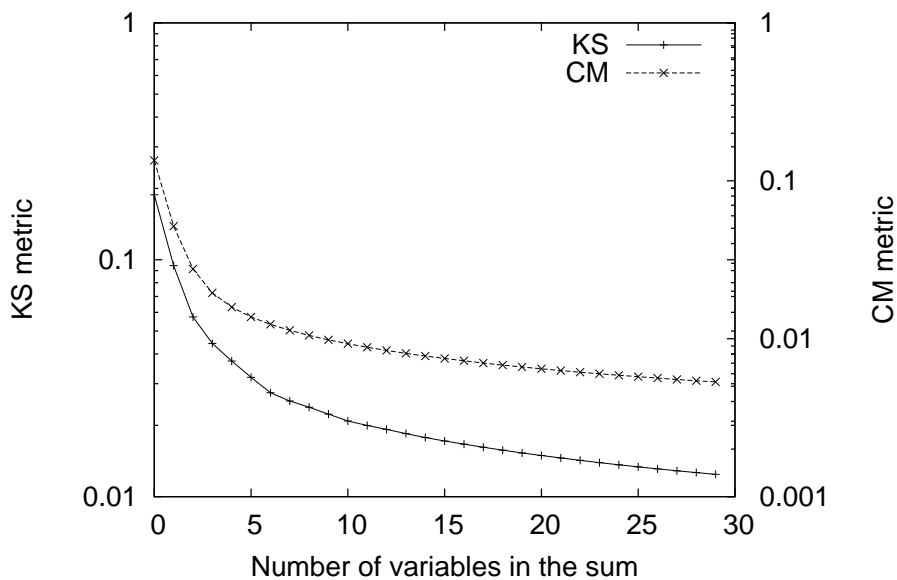
Figure 8: Precision when approximating the special distribution n -times by a normal distribution after n -sums with itself using the Kolmogorov-Smirnov and the Cramér-von-Mises metrics
