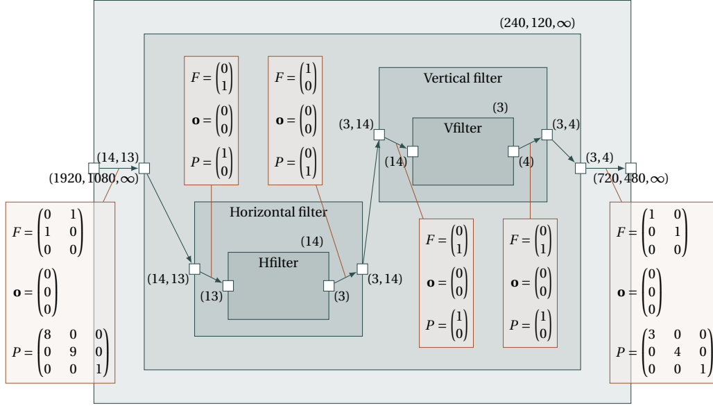
A hierarchical level has been created that is repeated (240, 120, \infty) times. The intermediate array between the filters has been reduced to the minimal size that respects the dependencies. If the inserted level is executed sequentially and if the two filters are executed on different processors, the execution can be pipelined.
