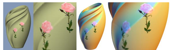
Figure 4: Topology-free painting with up-sampling. Left: The integration of bitmaps in the low resolution model (100k samples) can be done either by coloring existing surfels (left rose) or locally up-sampling the model to reach the brush resolution (right rose). Right: The high resolution mesh (7M polygons) textured with the edited point set. Note the difference in sharpness between the two roses, when the up-sampling is performed.
