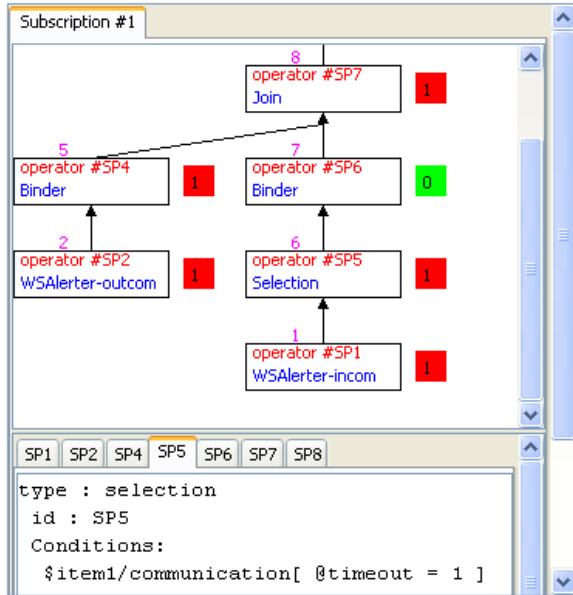
Fig. 4. Graphical user interface snapshot
