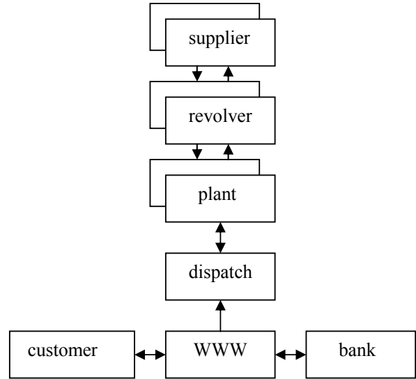
Fig. 5. Architecture of the example
