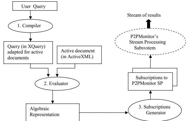
Fig. 2. Query Processing Subsystem
