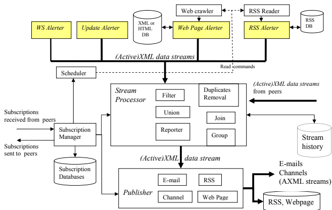
Fig. 1. Stream Processing Subsystem
