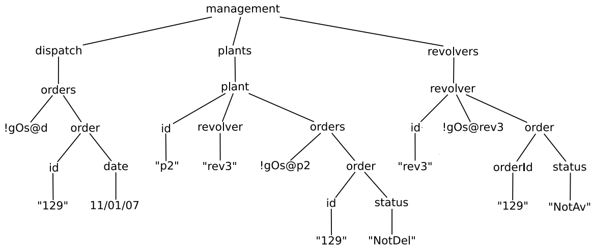
Fig. 6. An active document with streams
